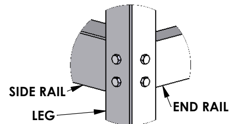
DETAIL B BLOWN UP VIEW OF LOWER JOINT
