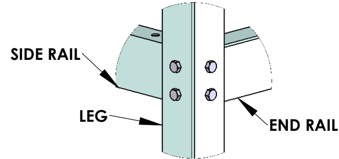
DETAIL B BLOWN UP VIEW OF LOWER JOINT (SIDE RAIL BOLTS ON INSIDE OF LEG OVER-LAPPING END RAIL. END RAIL BOLTS ON INSIDE OF LEG UNDER-LAPPING SIDE RAIL.)
