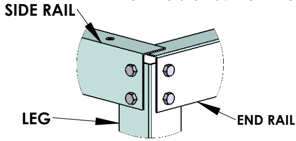
DETAIL A BLOWN UP VIEW OF TOP JOINT (SIDE RAIL BOLTS ON OUTSIDE OF LEG OVER-LAPPING END RAIL. END RAIL BOLTS ON OUTSIDE OF LEG UNDER-LAPPING SIDE RAIL.)
